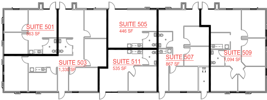
3 BUILDING 500 SCALE 1/8"=1'-0" 4,900 SF
